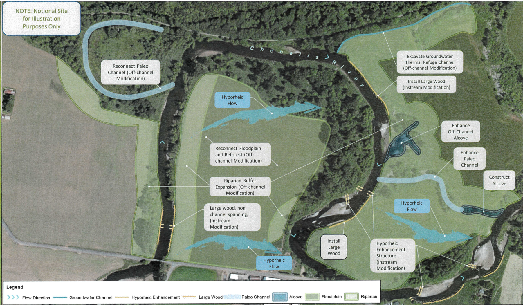
Chehalis Mitigation Conceptual Design - #2 Main Stem - Chehalis River Lewis County, WA
