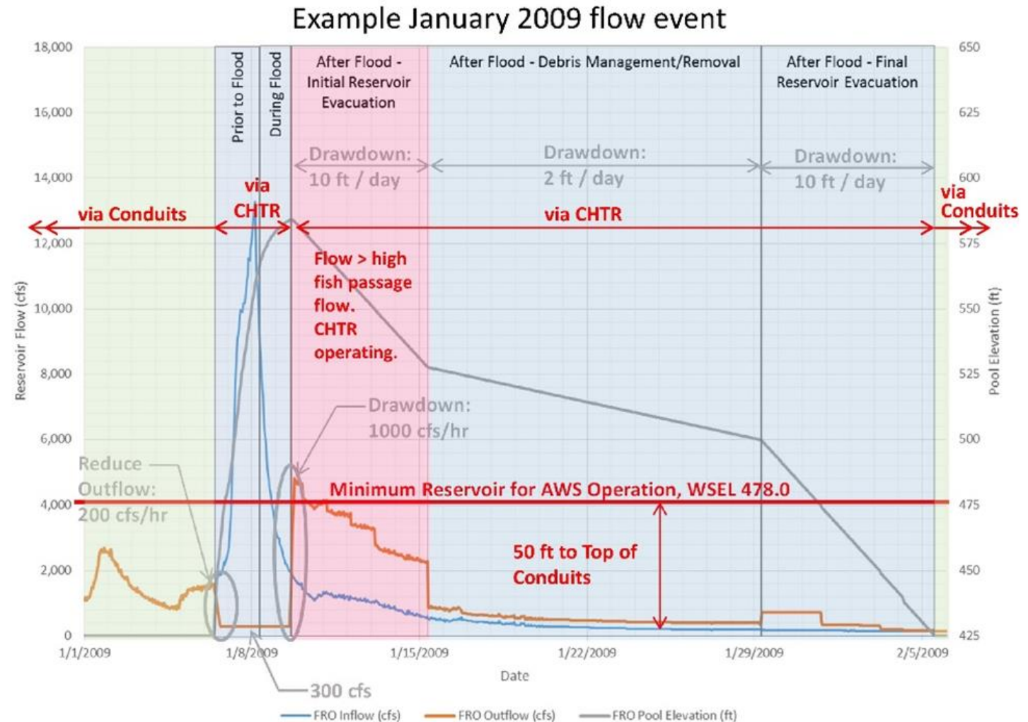
Potential Operation Overlaid on 2009 Flow Event Hydrograph
