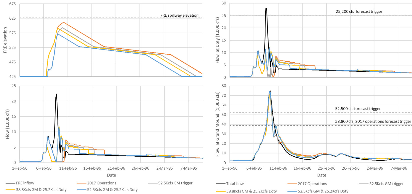
Figure 14-5. Forecast Trigger Analysis Results: February 1996 Event
