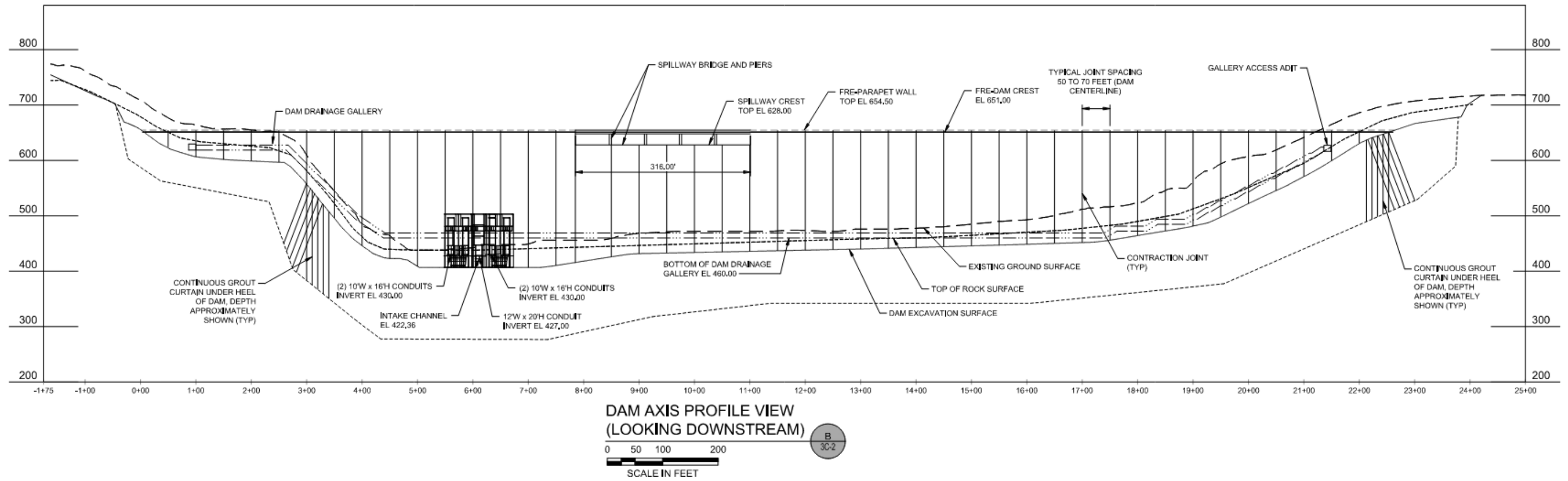
Figure 10-2. Profile View along FRE Dam Axis
