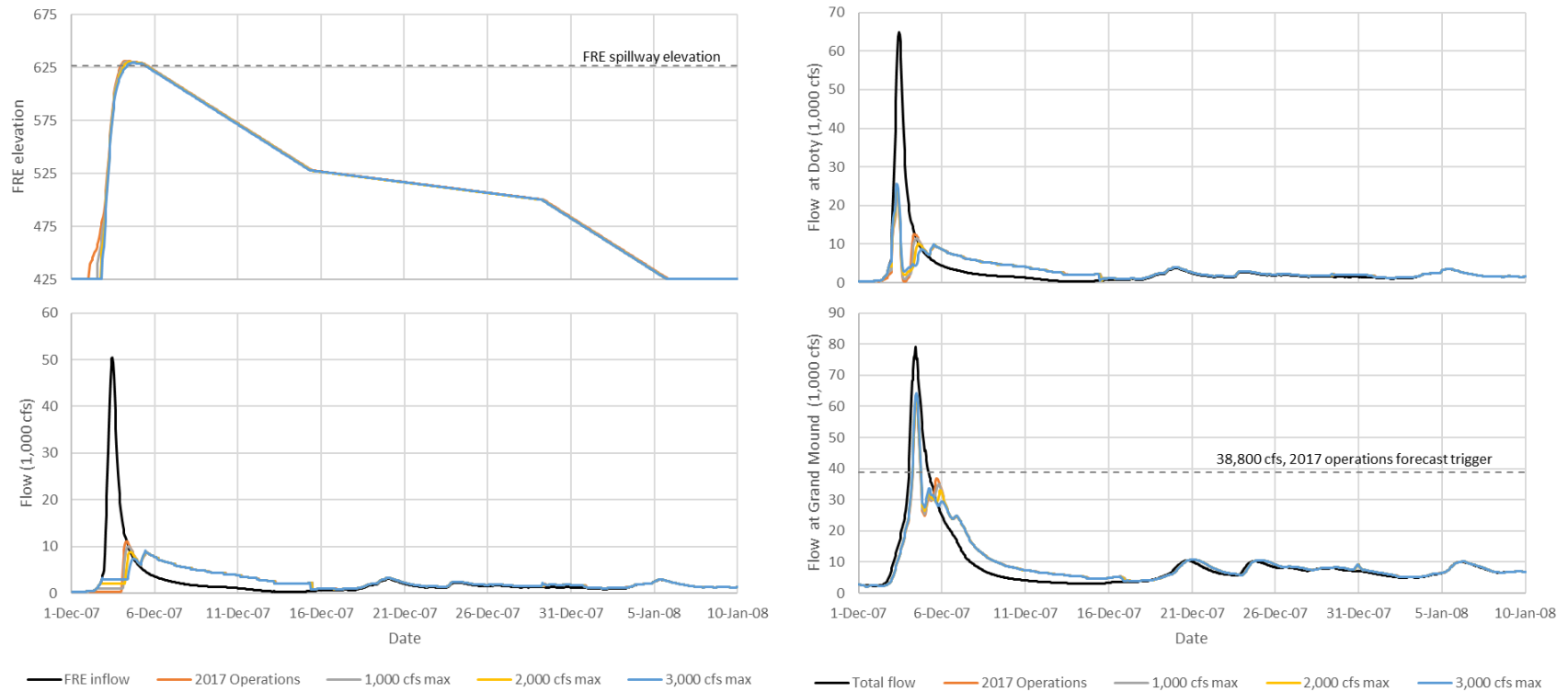
Figure 14-3. Maximum Release Sensitivity Analysis Results: December 2007 Event
