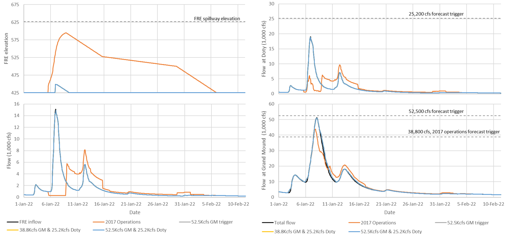
Figure 14-7. Forecast Trigger Sensitivity Analysis Results: January 2022 Event
