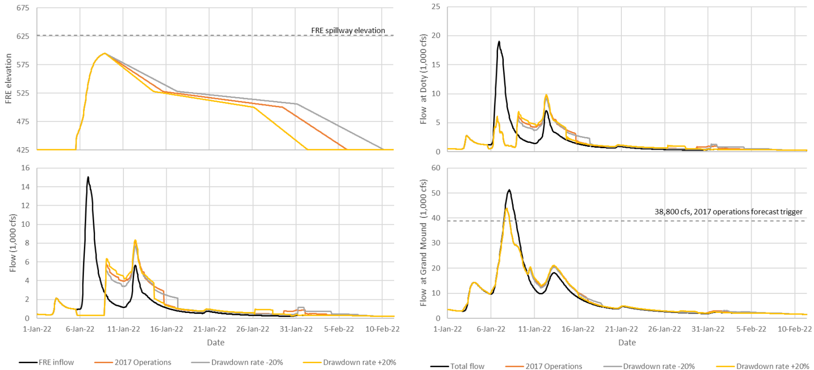
Figure 14-10. Drawdown Rate Sensitivity Analysis Results: January 2022 Event
